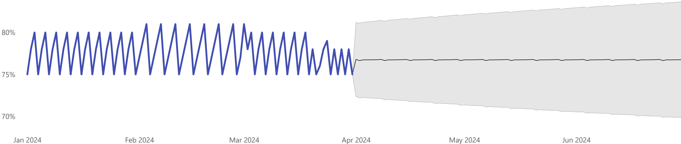
Forecasted Occupancy Trend - Q2 2024
