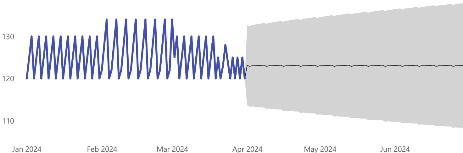
Forecasted ADR Trend - Q2 2024
